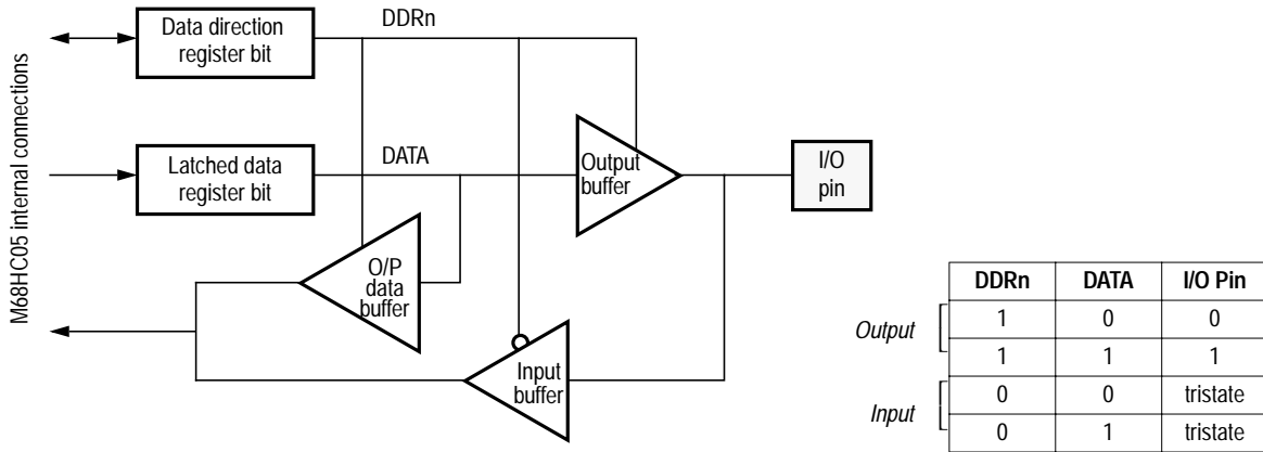
Figure 6-1 Standard I/O port structure
