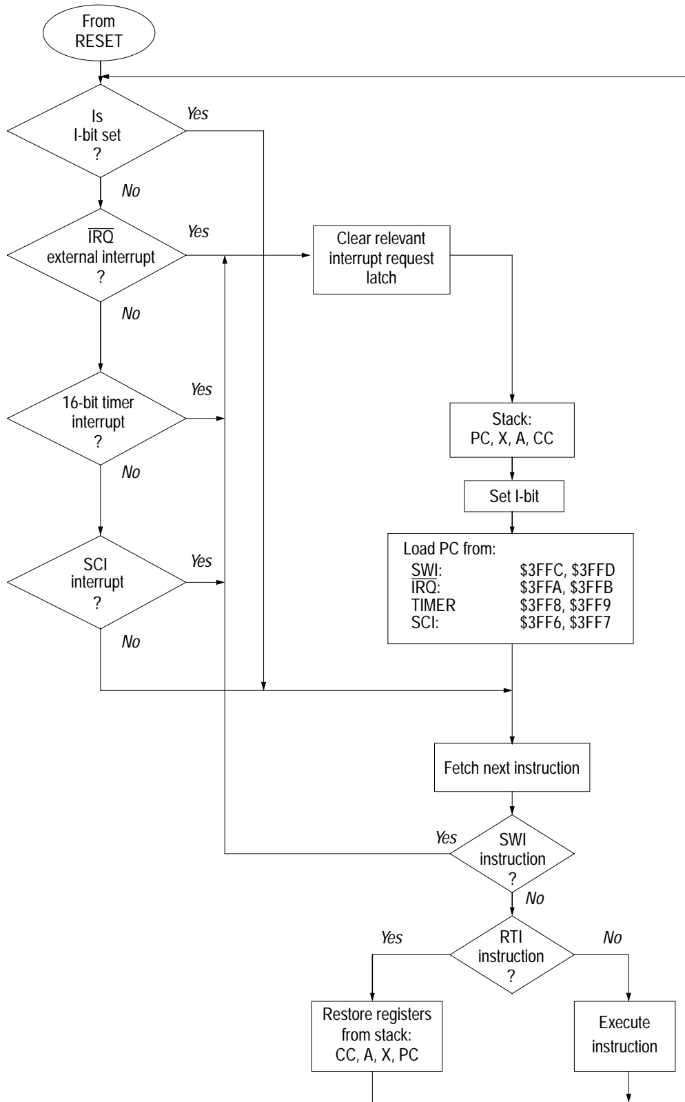
Figure 4-2 Interrupt flowchart
