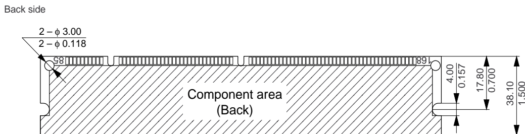
Detail A
